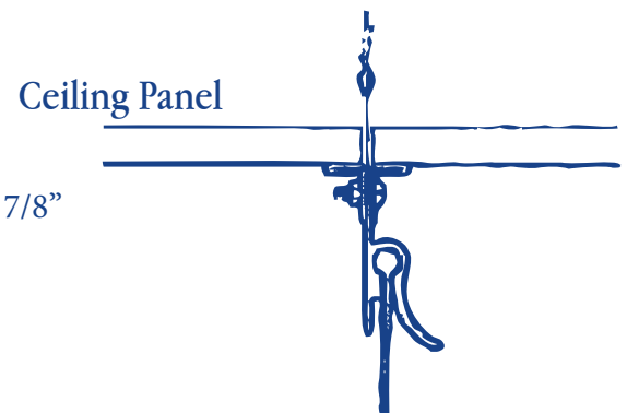
Suspended T-Bar Ceiling Mount
